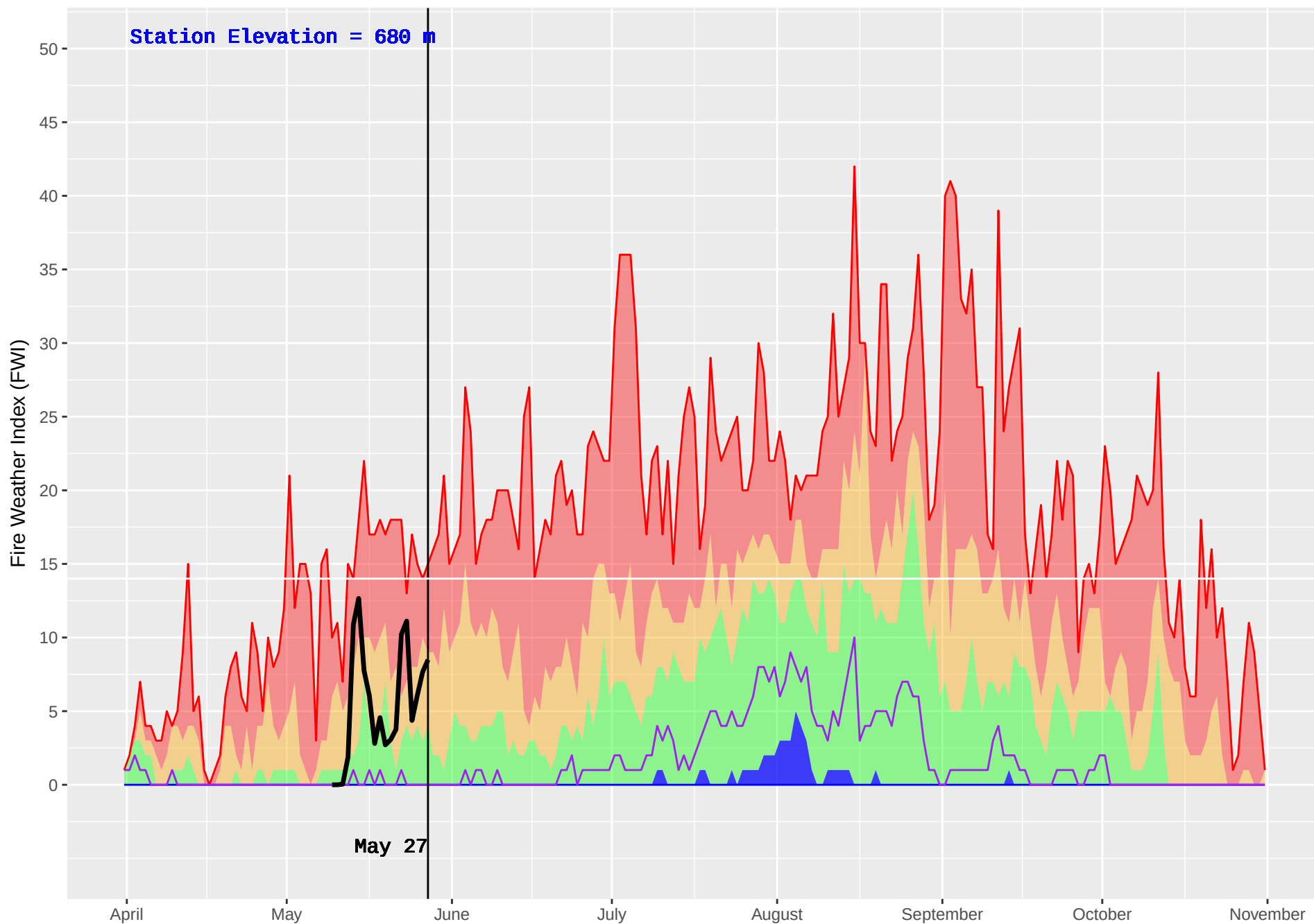
SUMMIT (11) : Historical (1985–2016) and Current (2018) Noon Fire Weather Index (FWI)
