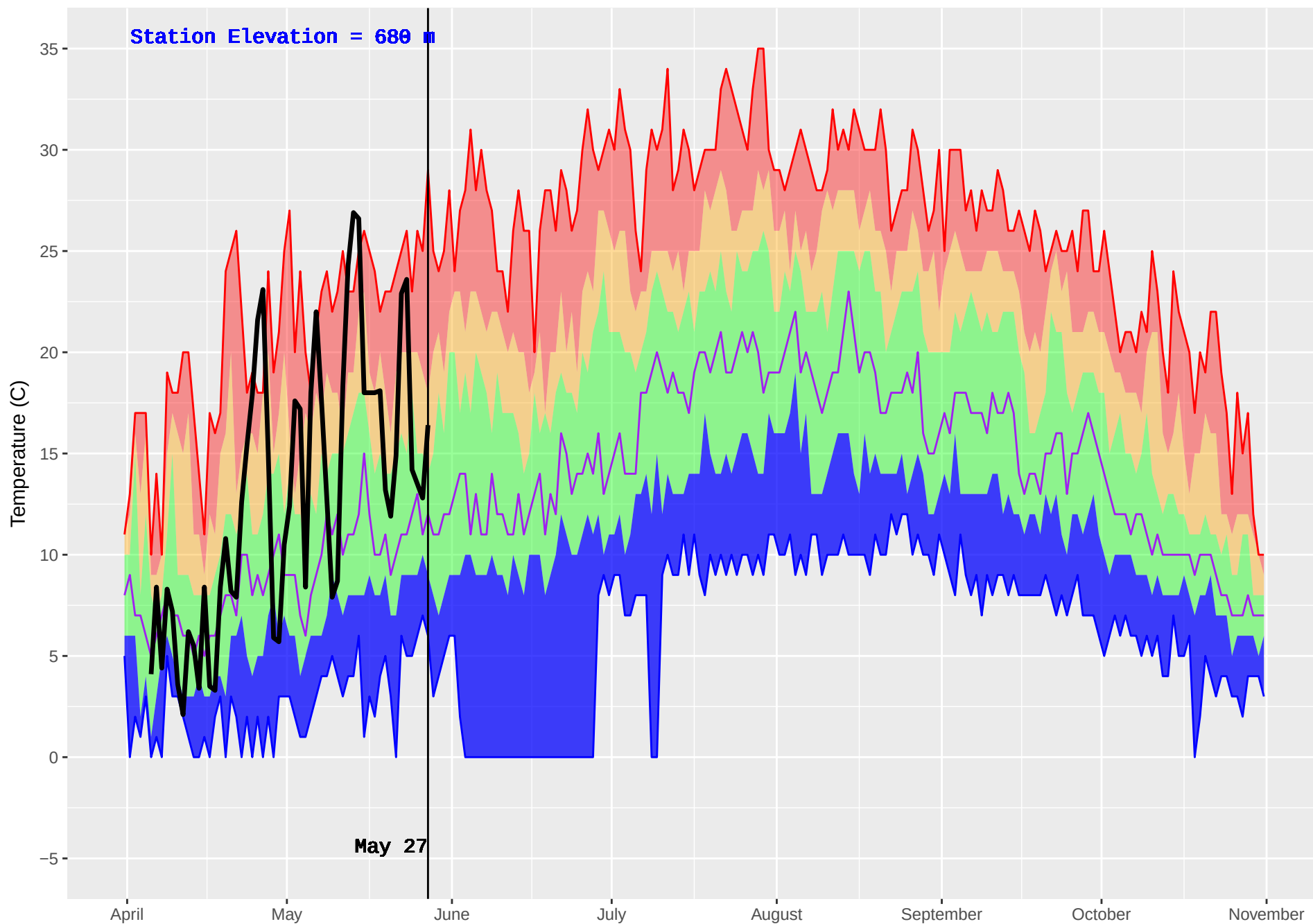
SUMMIT (11) : Historical (1985–2016) and Current (2018) Noon Temperature
