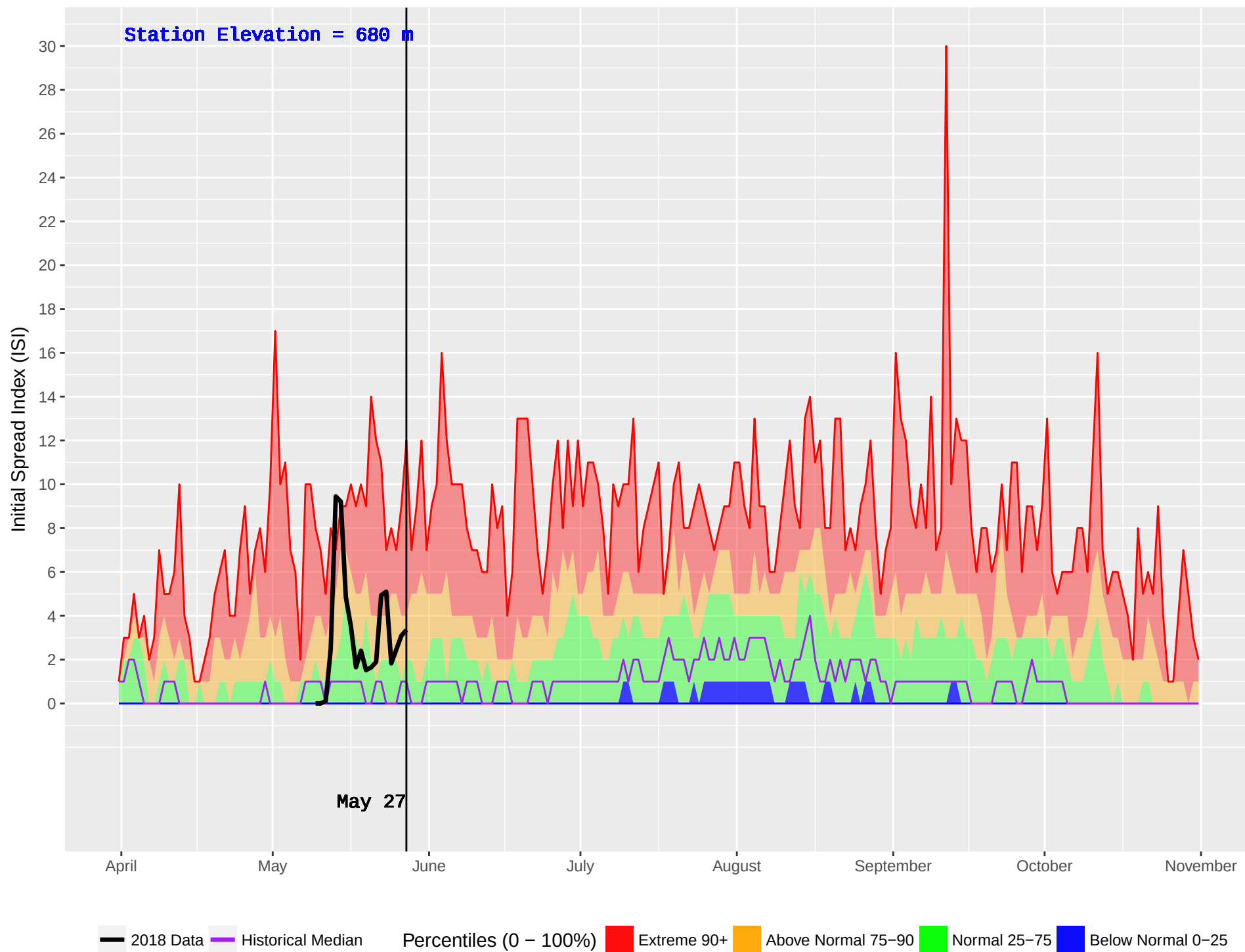
SUMMIT (11) : Historical (1985–2016) and Current (2018) Noon Initial Spread Index (ISI)
