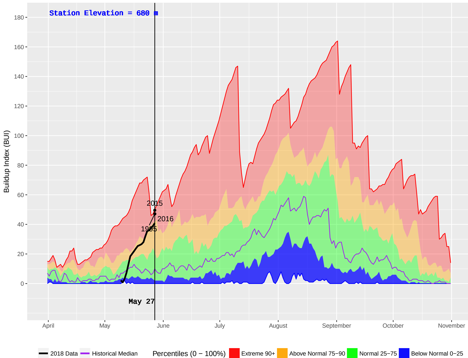
SUMMIT (11) : Historical (1985–2016) and Current (2018) Noon Buildup Index (BUI)
