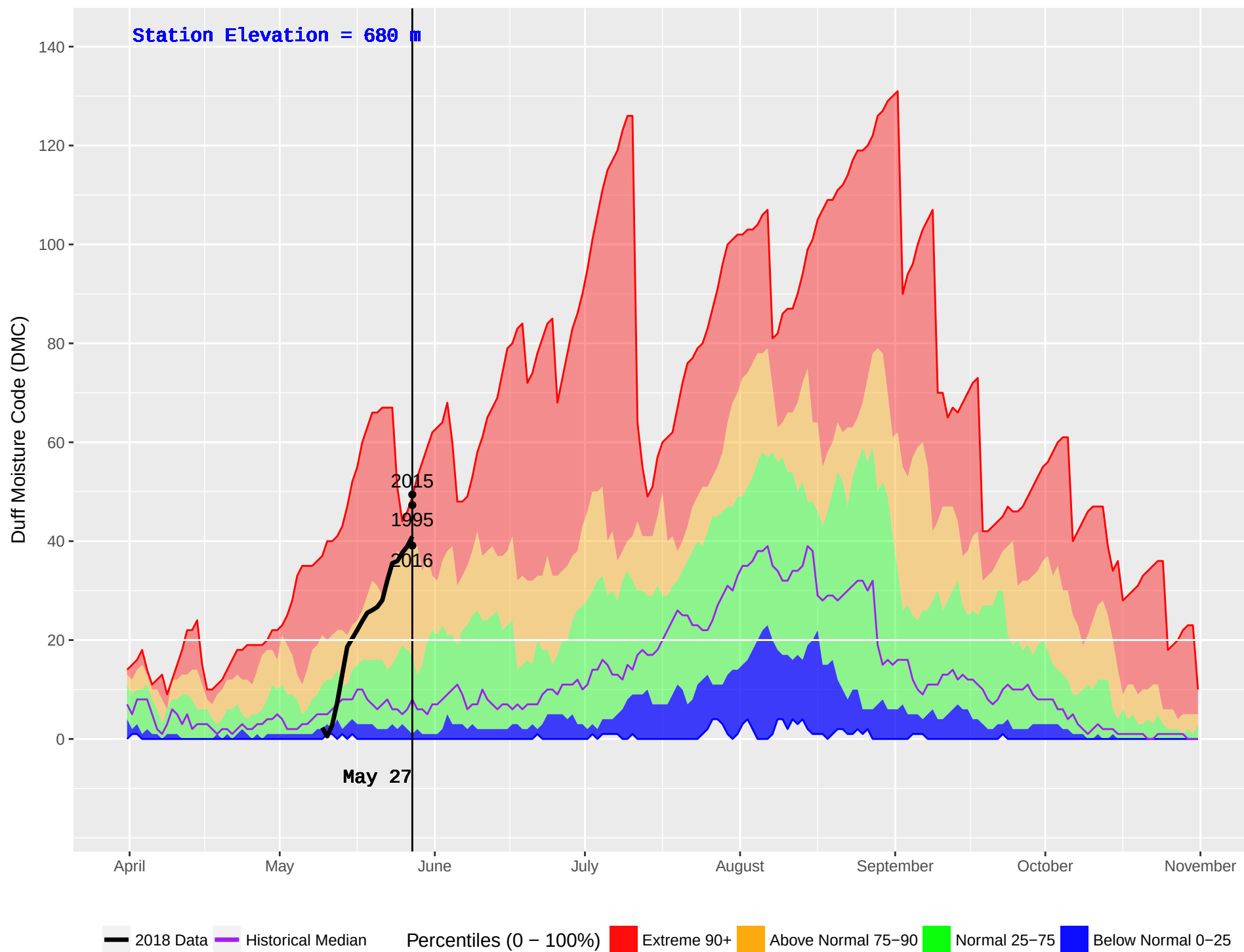
SUMMIT (11) : Historical (1985–2016) and Current (2018) Noon Duff Moisture Code (DMC)
