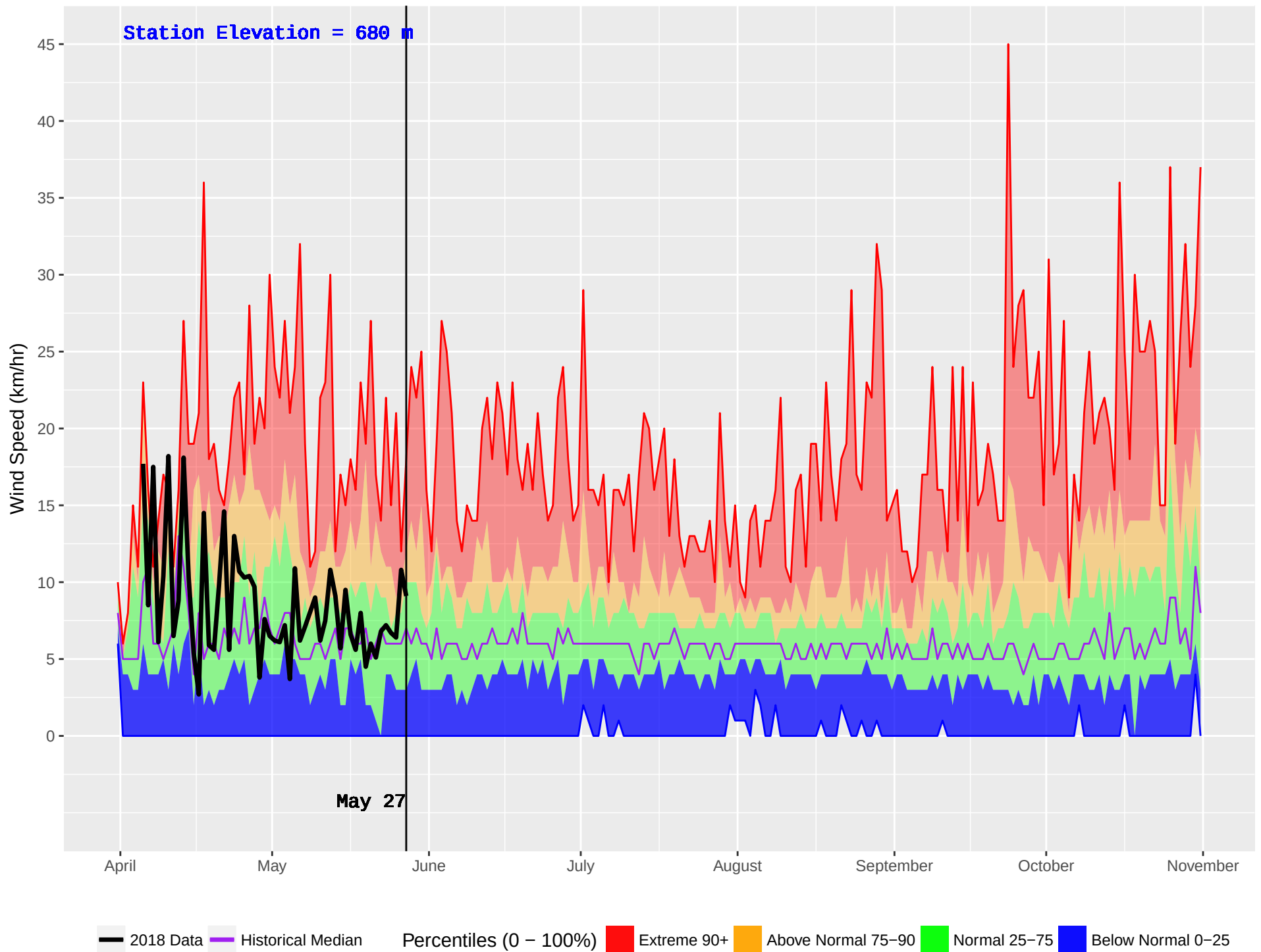
SUMMIT (11) : Historical (1985–2016) and Current (2018) Noon Wind Speed
