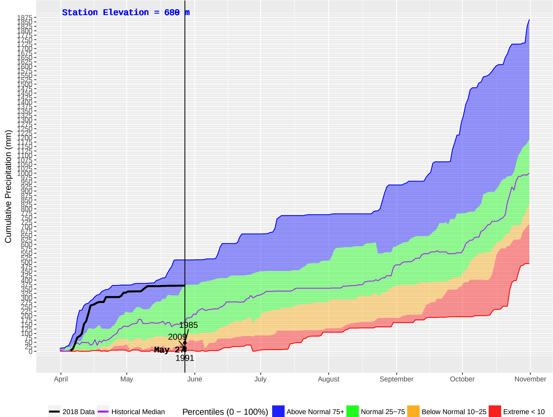
SUMMIT (11) : Historical (1985–2016) and Current (2018) Noon Cumulative Precipitation
