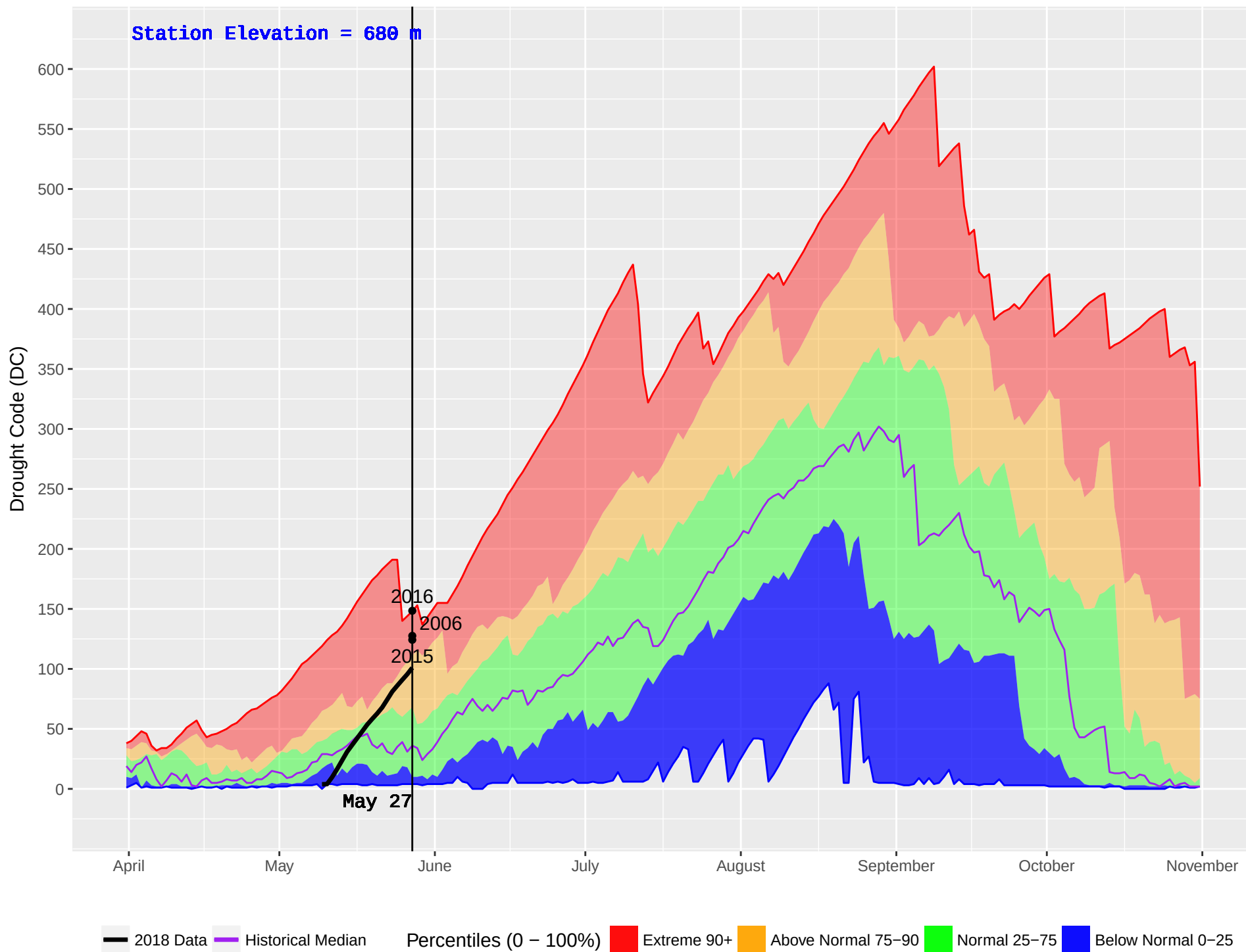
SUMMIT (11) : Historical (1985–2016) and Current (2018) Noon Drought Code (DC)
