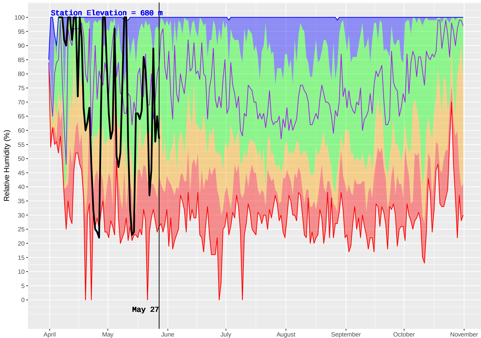
SUMMIT (11) : Historical (1985–2016) and Current (2018) Noon Relative Humidity
